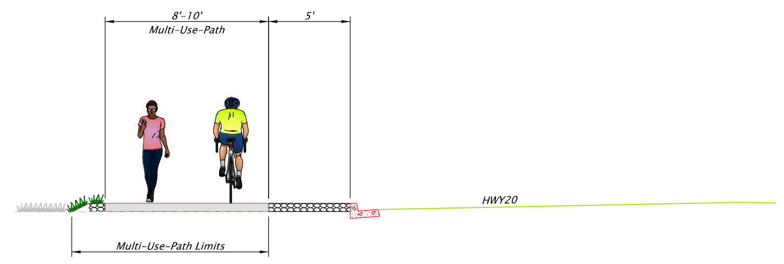
ASBAHR TO PILKINGTON TYPICAL SECTION
