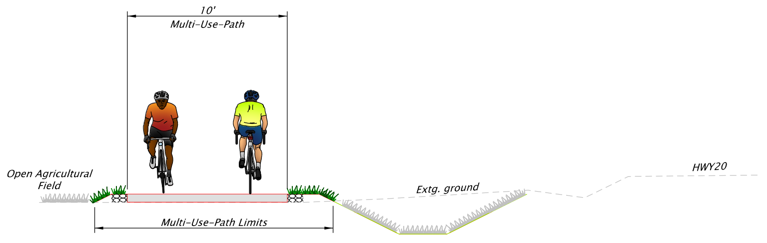
MERLOY TO ASBAHR TYPICAL SECTION
