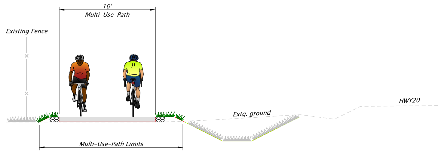
MERLOY TO ASBAHR TYPICAL SECTION
