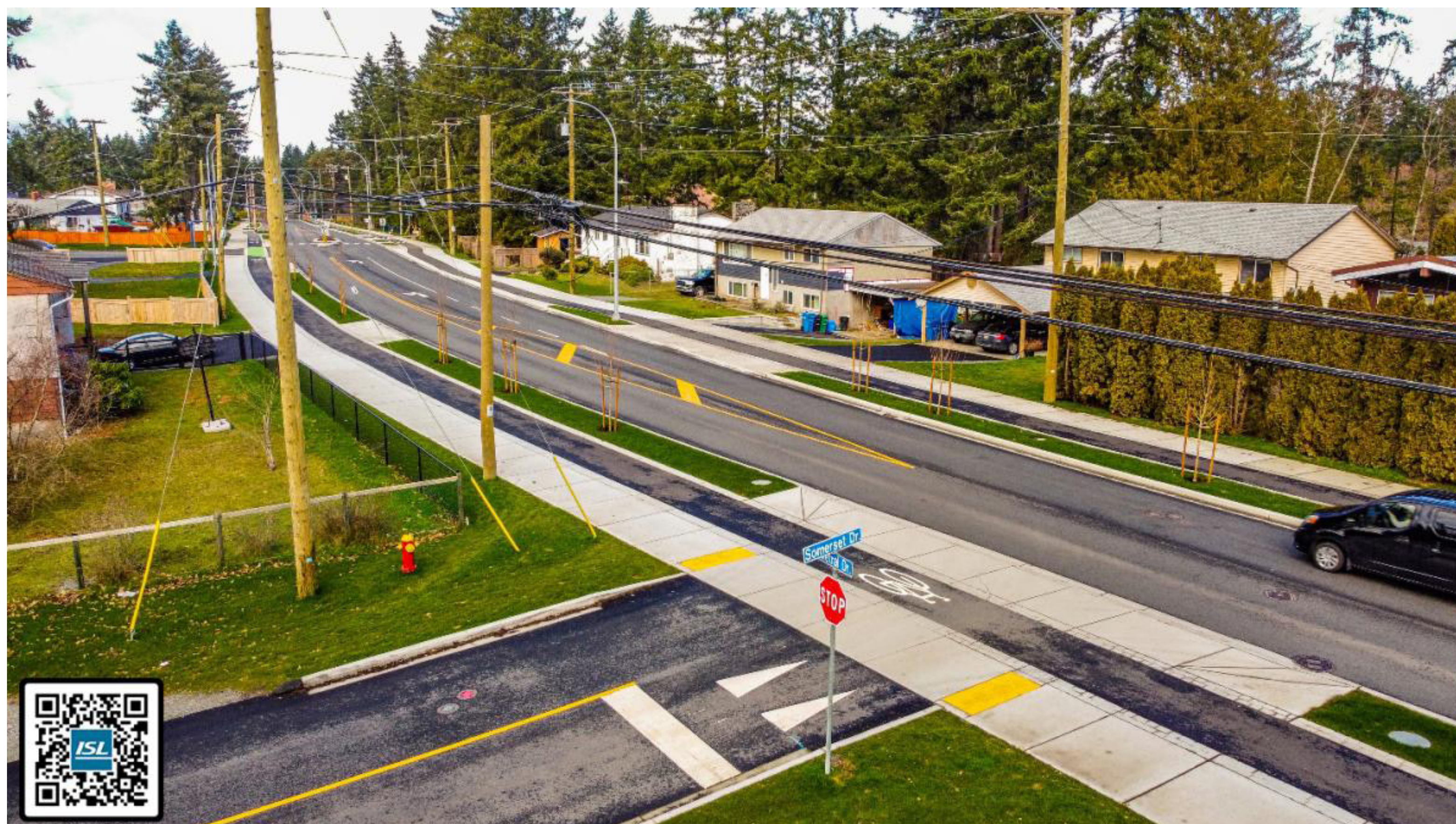
Aerial View of a Raised Pedestrian and Bicycle Crossing at a Side Street
